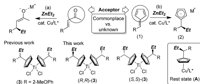
Scheme 1. Common \text{Cu}^{\text{I}} -catalyzed asymmetric 1,4-addition (a) vs. unknown carbocycloaddition (b) reactions, and applications.
