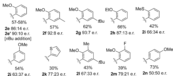
Scheme 2. Scope of catalytic cupration of fulvenes ( 1 ) as a function of 6-aryl unit.
